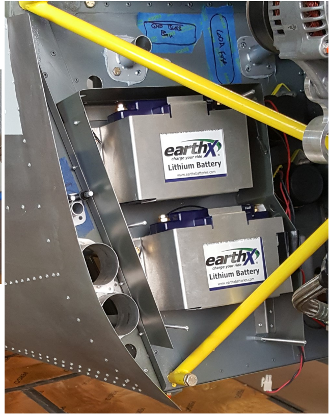
Cool air box for dual Earth-X lithium batteries—minus cover
